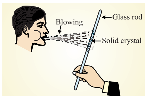
Fig. 12.3 : Testing of crystallization point
