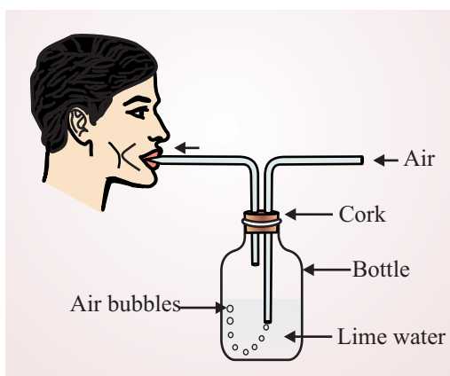
Fig. 15.1 : Testing presence of \text{CO}_2 in air
