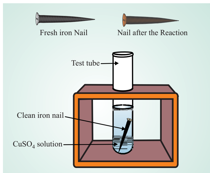
Fig. 20.3 Displacement reaction between iron and \text{CuSO}_4 Solution
