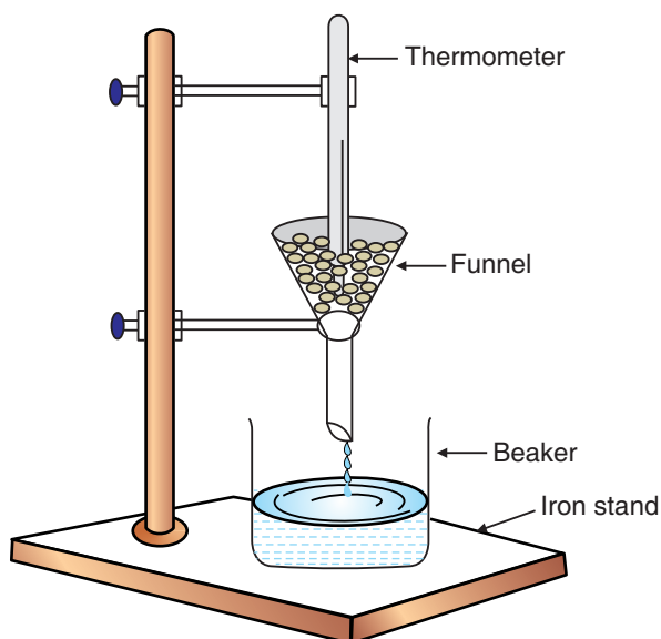
Fig. 5.1: Experimental set up for finding melting point of ice
