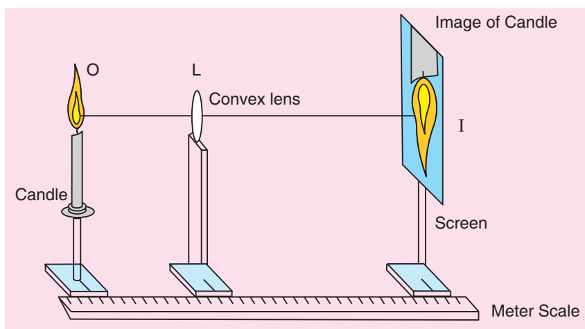
Fig. 7.1: Setting of the experiment for convex lens.
