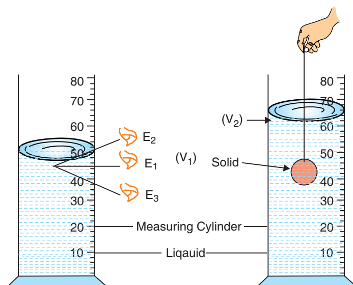
Fig. 1.2: Reading level of liquid in a measuring cylinder
