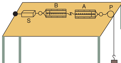
Fig. 4.1: Experimental set-up
