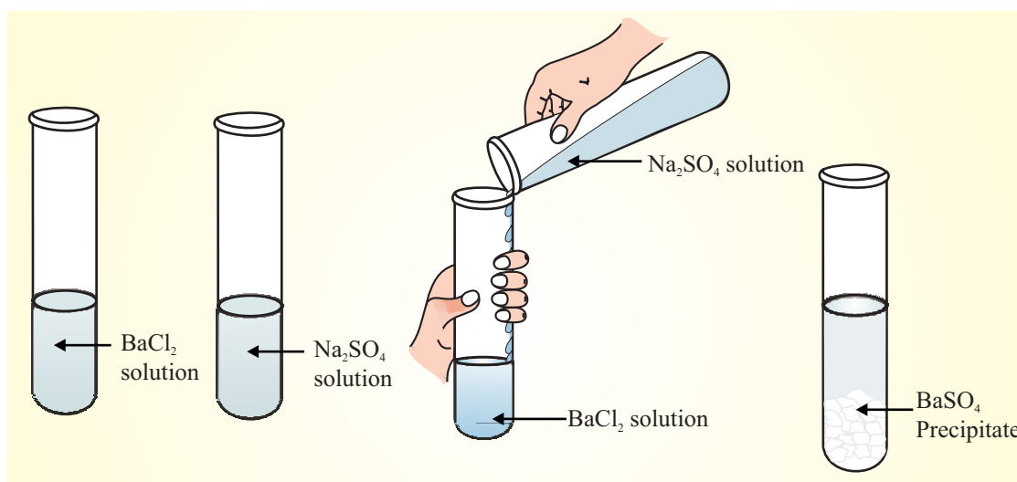
Fig. 20.4 Double displacement reaction between BaCl_2 and Na_2SO_4
