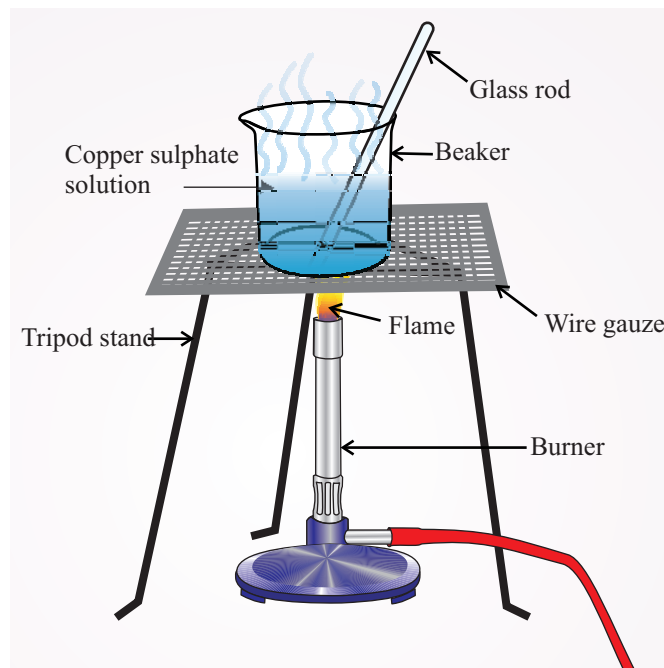
Fig. 12.2 : Concentration of the solution by heating
