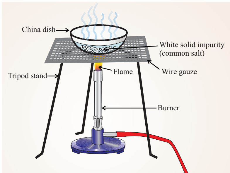
Fig. 12.1 Evaporation
