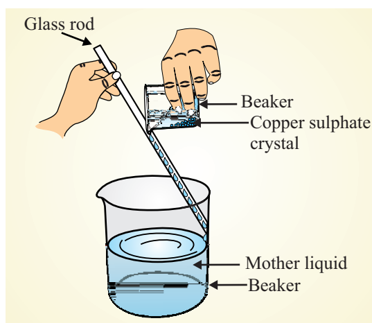
Fig. 12.5 : Decanting off the mother liquor
