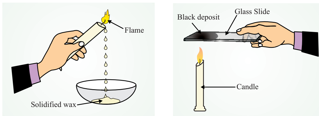
Fig. 13.1 : (a) Physical change
