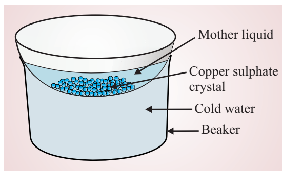
Fig. 12.4: Cooling the concentrated solution undisturbed for 4-5 hrs to obtain crystals
