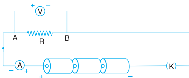
Fig. 8.2 (c) Circuit Diagram with three cells
