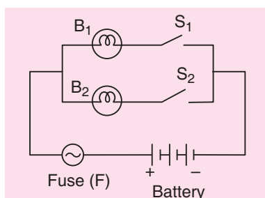
Fig. 9.1 Circuit diagram for household circuit
