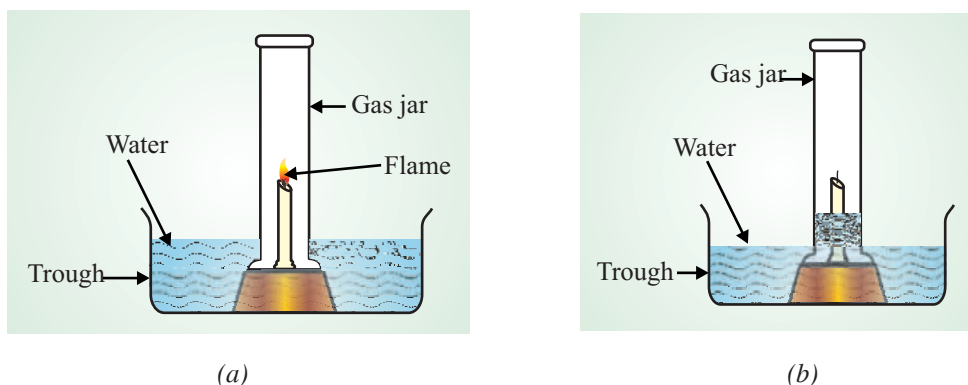
Fig. 16.1 : Showing presence of oxygen in air(a) Before (b) After
