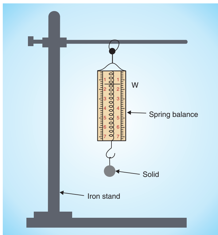
Fig. 1.1: Determination of mass of solid using spring balance
