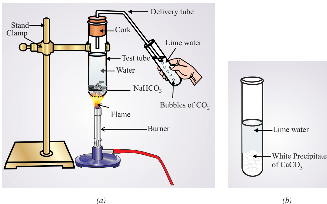
Fig. 19.1: (a) Heating of baking soda and passing the \text{CO}_2 produced through lime water (b) Formation of white ppt. of \text{CaCO}_3
