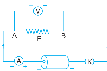
Fig. 8.2 (a) Circuit Diagram with single cell
